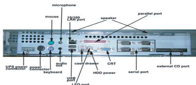
JIVA 8000 Main Board Interface Diagram
